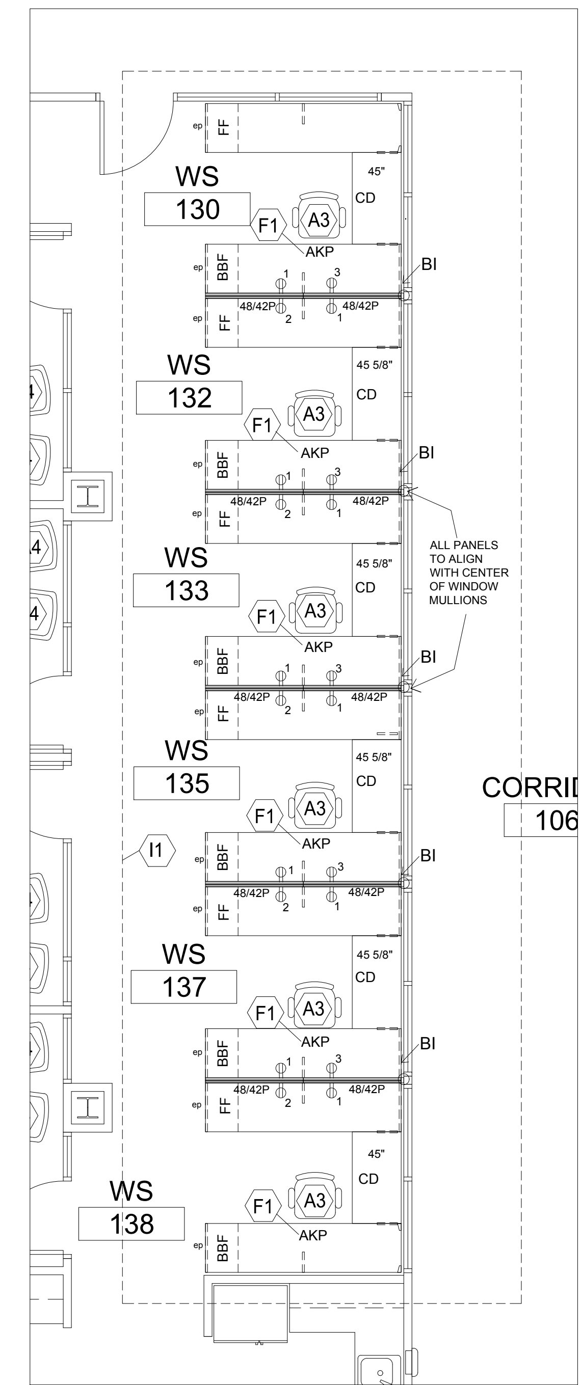
11 WORKSTATIONS ENLARGED PLAN SCALE: 1/4" = 1'-0"
